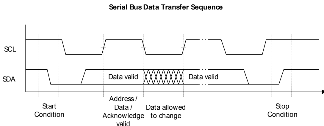
Figure 5.3: Data transfer on the serial bus
