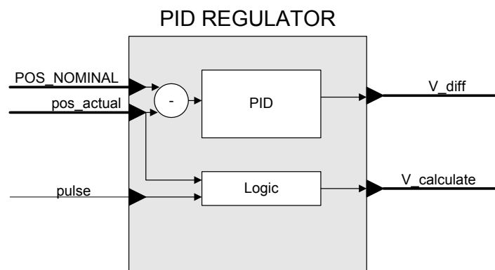
Figure 10.1: Simplified schematic the PID controller
