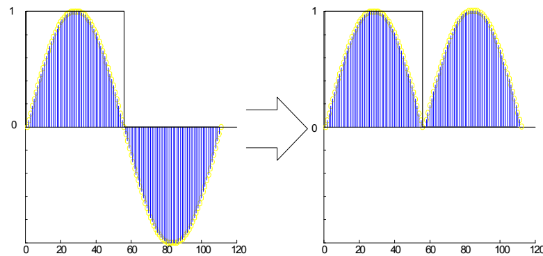
Figure 9.5: Derivation of the phase polarity in sine step mode
