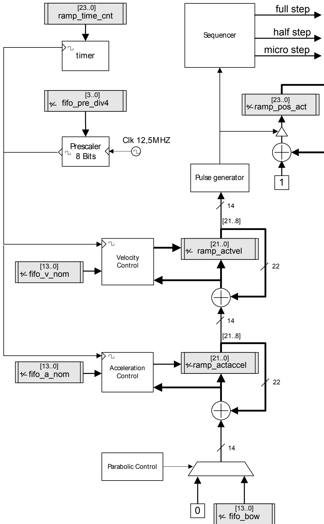
Figure 7.1: Schematic of the ramp generator
