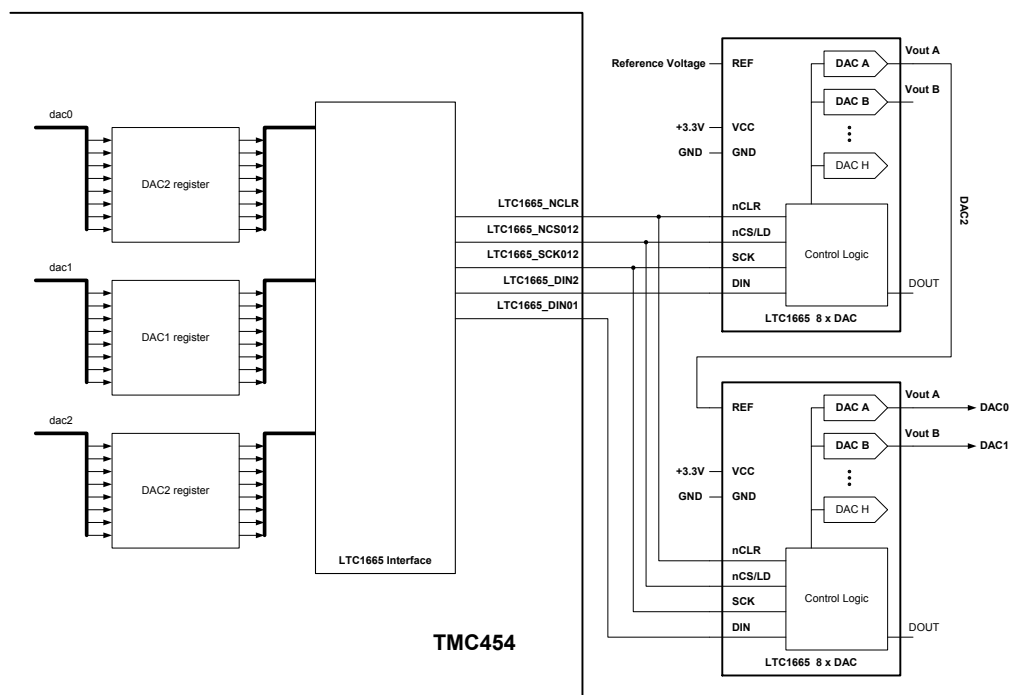
Figure 4.3: Connection of external DACs LTC1665 with the TMC454
