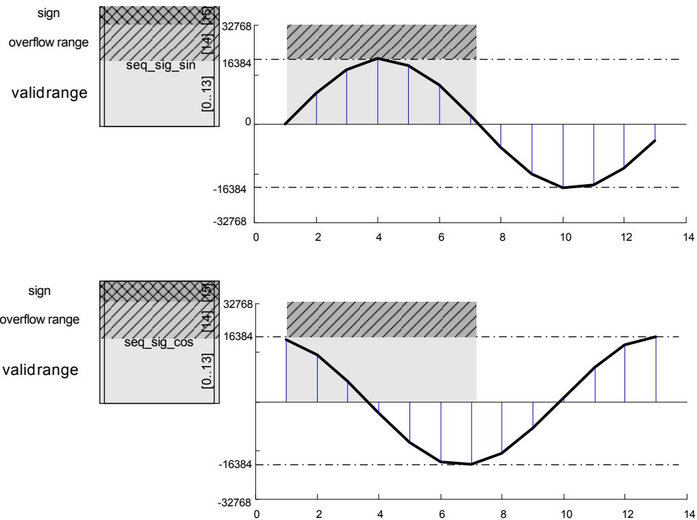
Figure 9.1: Range for sine wave and cosine wave.
