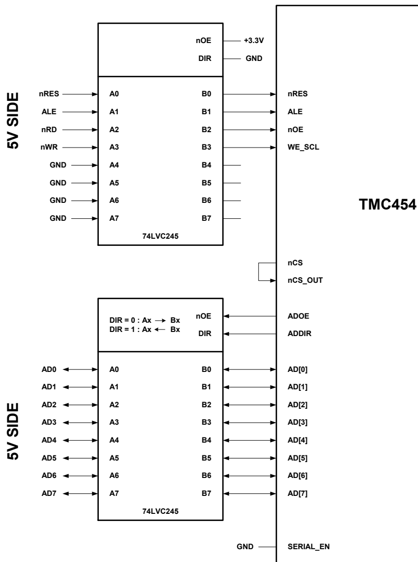
Figure 5.1 : Parallel Interface with 5V to 3V3 Level Shifters
