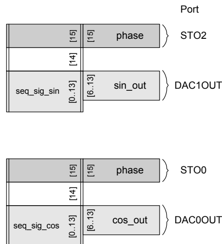
Figure 9.6: Output mapping in sine step mode
