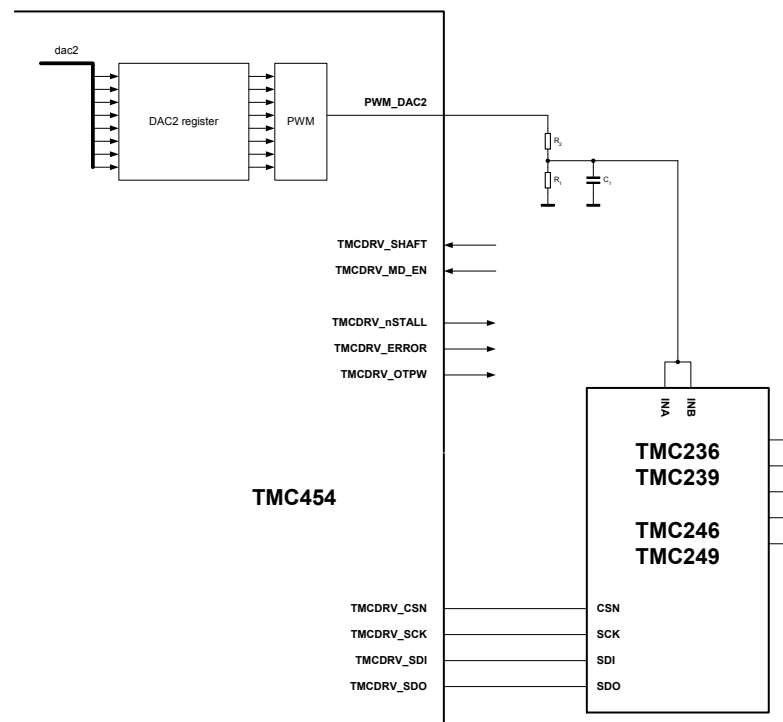
Figure 4.2 : Connection of a TRINAMIC driver with the TMC454
