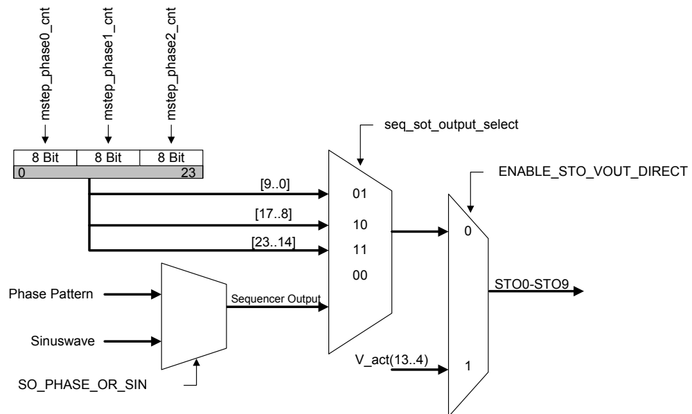
Figure 9.12: Control of the digital outputs STO0-STO9
