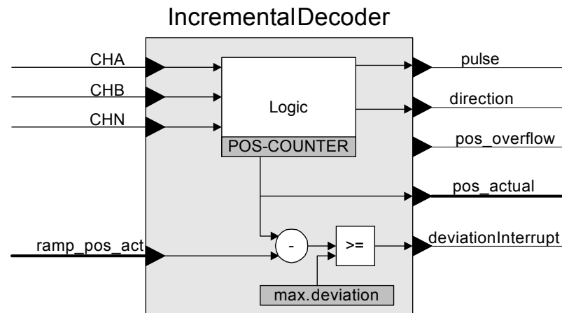
Figure 8.1: Schematic of the Incremental Encoder Interface
