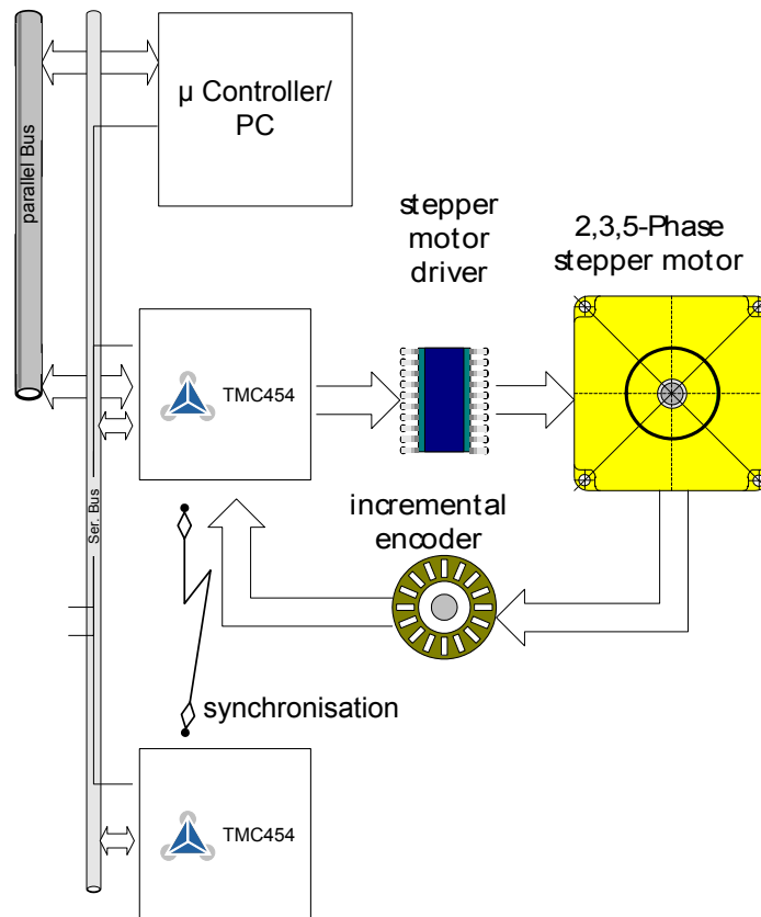
Figure 2.1: System environment of the TMC454
