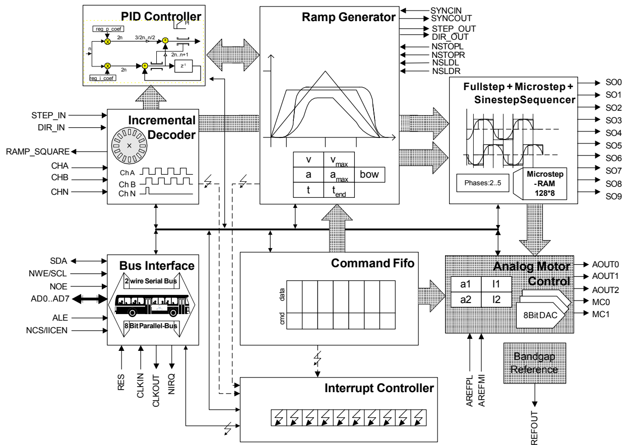
Figure 3.1: Block diagram of the TMC454's modules
