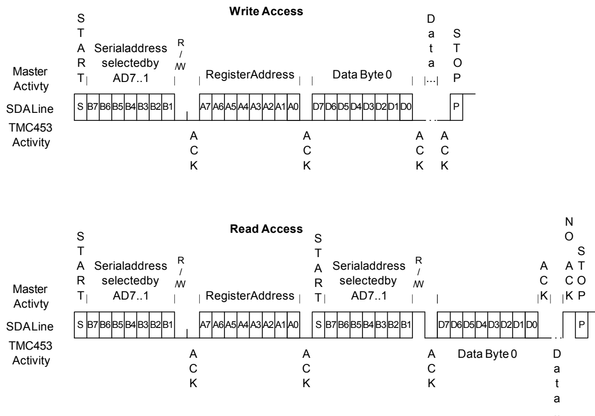
Figure 5.4: Telegram on the serial bus
