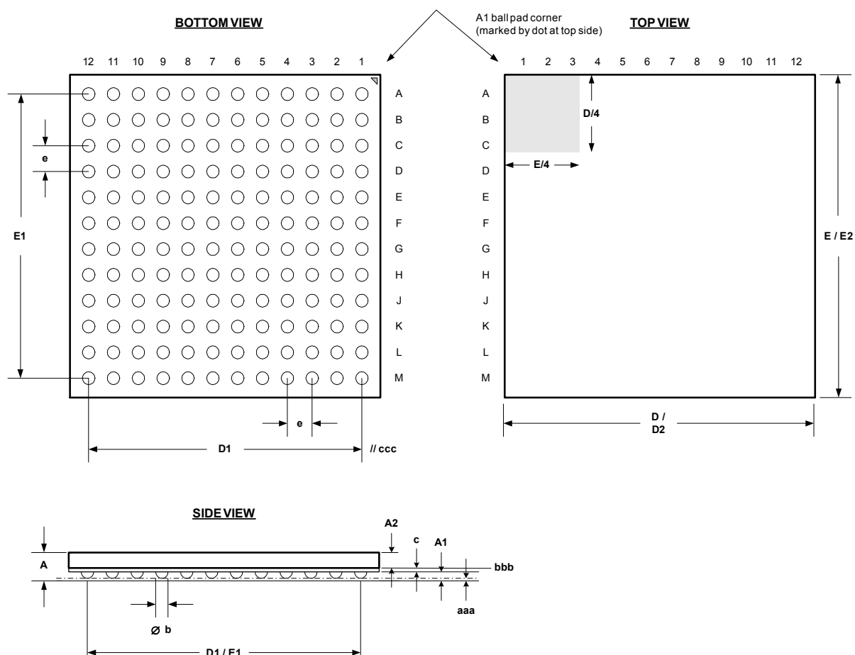
Figure 4.1 – Package Outline Drawing FBGA144 – MO-192 VAR DAD-1
