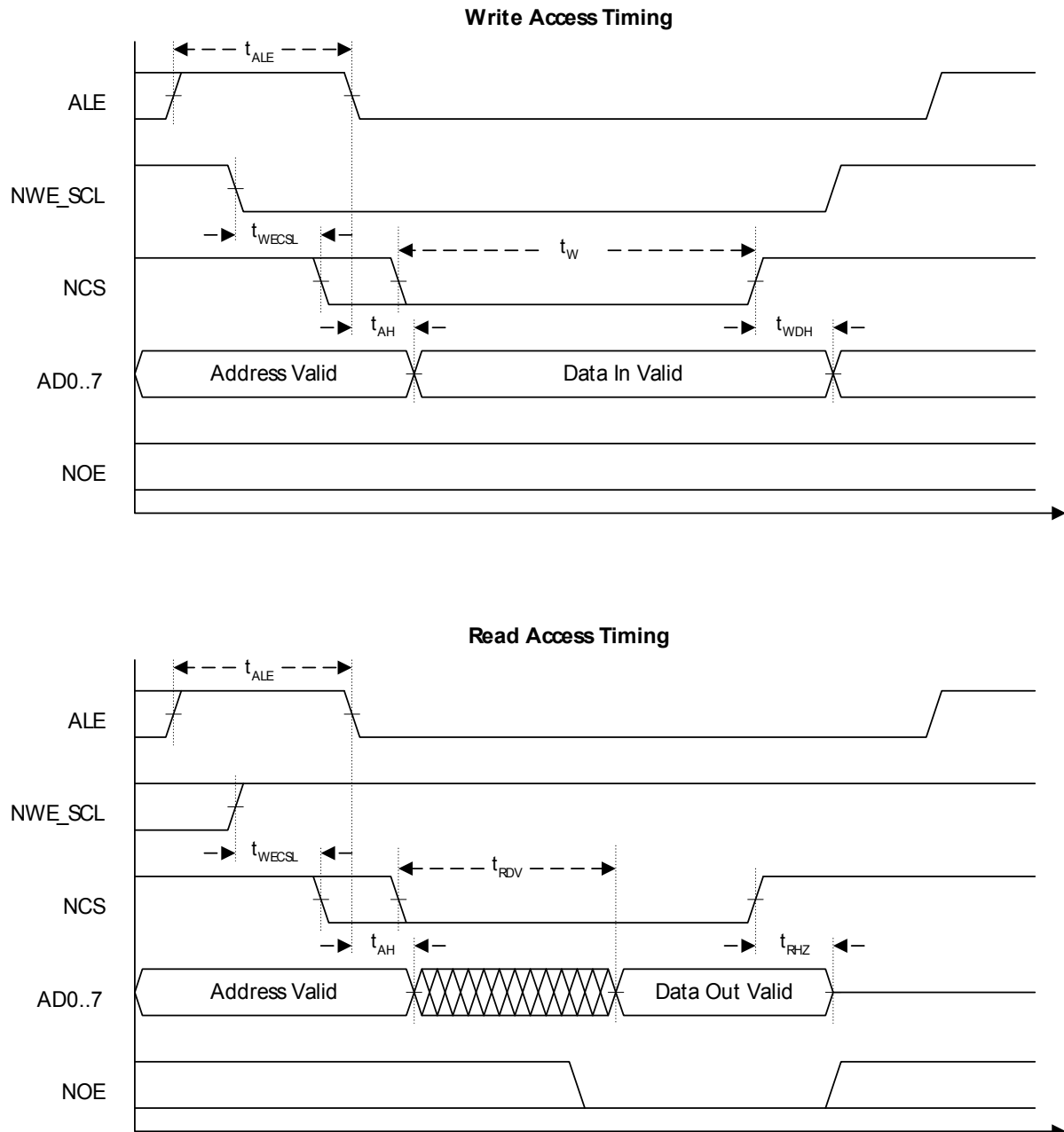
Figure 5.2: Timing of the parallel interface
