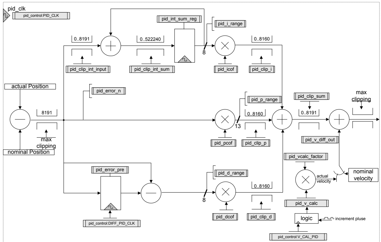
Figure 10.2: PID controller and registers
