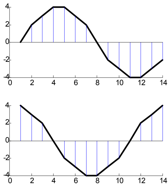
Figure 9.3: Amplitude vs. step number. Near sine curve with k=1 and S_n-C_n = 4
