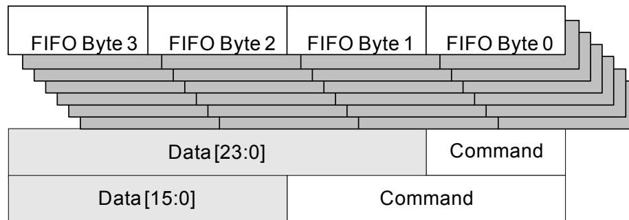
Figure 6.1: FIFO-Command types
