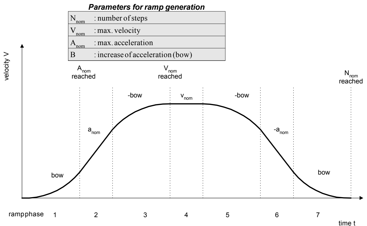
Figure 7.2: Automatically generated S-ramp
