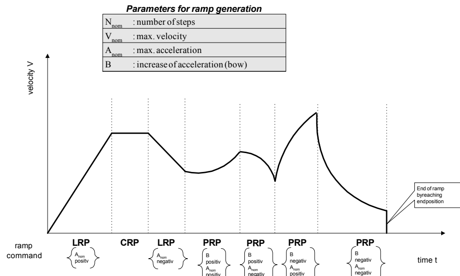
Figure 7.3: User defined ramp
