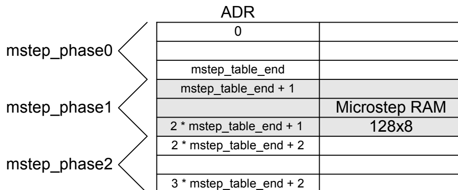
Figure 9.11: Organization of the microstep RAM when using three separate tables.
