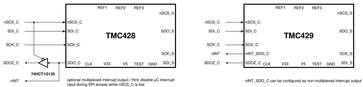
Figure 20.1 TMC428 SDO_C tristate output using a single gate 74HCT1G125. The TMC429 has a dedicated tristate output (SDOZ_C). nINT_SDO_C can be switched to nINT.
