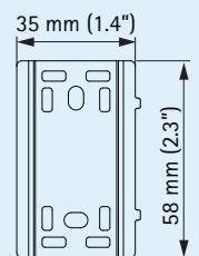
Mounting rail
