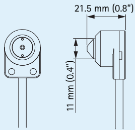
Sensor unit
