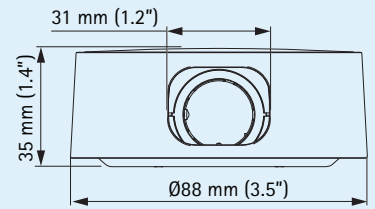
Outdoor housing
