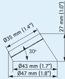
Angled mounting bracket
