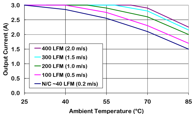
Figure 5. Output Current Derating vs Ambient Temperature & Airflow (converter mounted vertically with air flowing from pin 3 to pin 1, Vin = 62 V.)
