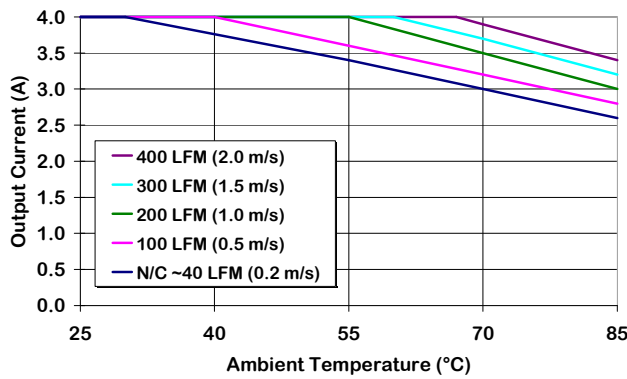
Figure 3. Output Current Derating vs Ambient Temperature & Airflow (converter mounted vertically with air flowing from pin 3 to pin 1, Vin = 12 V.)
