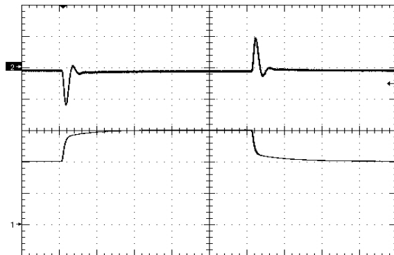
Figure 14. Load Transient Response (100mV/div), di/dt=0.5 A/uS, 50% - 75% - 50% of full load, 330uF low ESR tantalum, time scale: 200uS/div.
