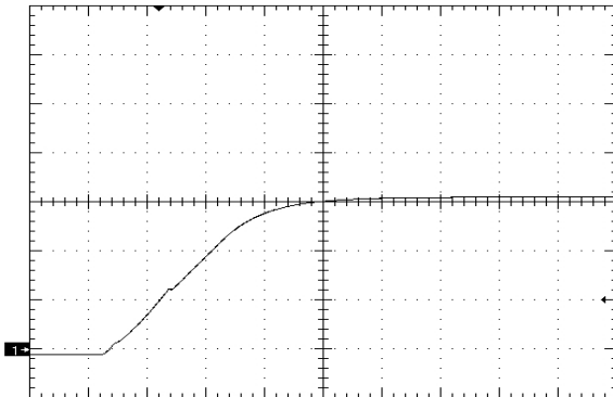
Figure 11. Startup Waveform via Enable Pin, time scale 4mS/div. Vin=Vin_nom, full resistive load (negative enable.)
