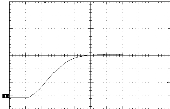
Figure 12. Startup Waveform via Enable Pin, time scale 4mS/div. Vin=Vin_nom, full resistive load + 10000uF (negative enable.)
