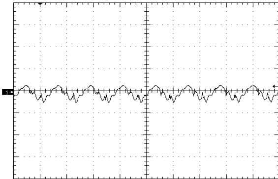
Figure 9. Output Voltage Ripple (20mV/div), time scale – 2uS/div. Vin=Vin_nom, full resistive
