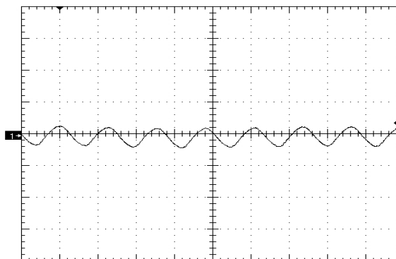
Figure 10. Input Reflected Ripple Current (10mA/div) time scale - 2uS/div. Vin=Vin_nom, full resistive
