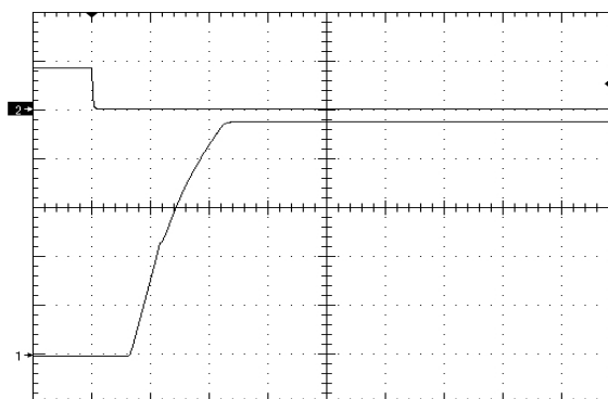
Figure 12. Startup Waveform via Enable Pin (5V/div), time scale 10mS/div. Vin=Vin_nom, full resistive load + 1000uF (negative enable.)
