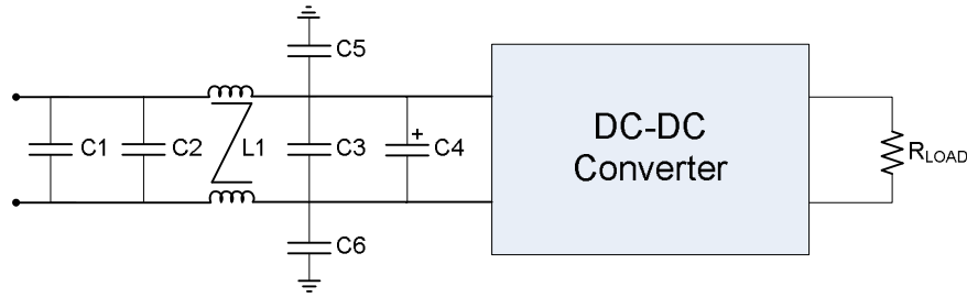
Figure 17. EMI Filter
