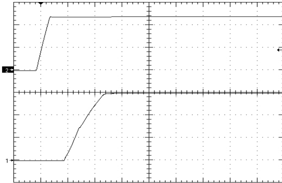
Figure 11. Startup Waveform via Line Voltage, time scale 10mS/div. Vin=Vin_nom, full resistive load
