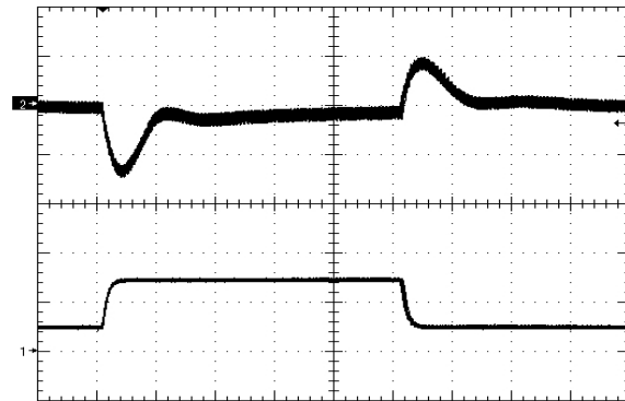
Figure 14. Load Transient Response (50mV/div), di/dt=0.25A/uS, 25% - 75% of full load, 2000uF Oscon low ESR, time scale: 200uS/div. Ch2 5A/div
