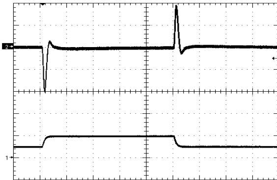
Figure 13. Load Transient Response (100mV/div), di/dt=0.1A/uS, 50% - 25% - 50% of full load, time scale: 200uS/div. Ch2 5A/div
