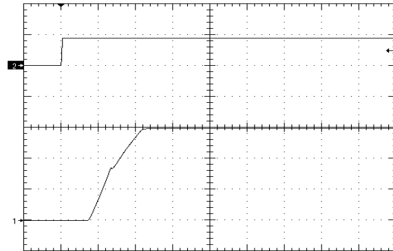
Figure 12. Startup Waveform via Enable Pin (5V/div), time scale 10mS/div. Vin=Vin_nom, No Load + 2200uF (positive enable.)
