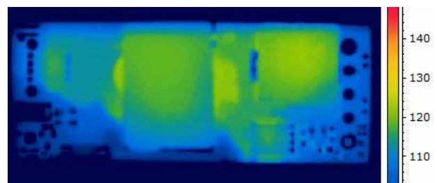
Figure 8. Thermal Image of CPE10C48 (10A output, 55C Ambient, 200lfm airflow, Vin = 48V, airflow from pin 3 to pin 1, T max = 123°C)
