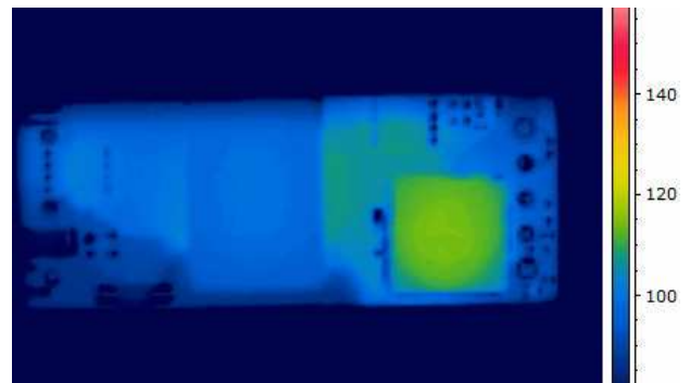
Figure 8. Thermal Image of CPE8B48 (8A output, 55C Ambient, 200lfm airflow, Vin = 48V, airflow from pin 3 to pin 1, T max = 114°C)
