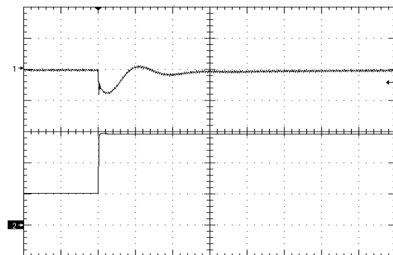
Figure 14. Load Transient Response (100mV/div), di/dt=3.0A/uS, 25% - 75% of full load, 2000uF Oscon low ESR across output, time scale: 200uS/div.
