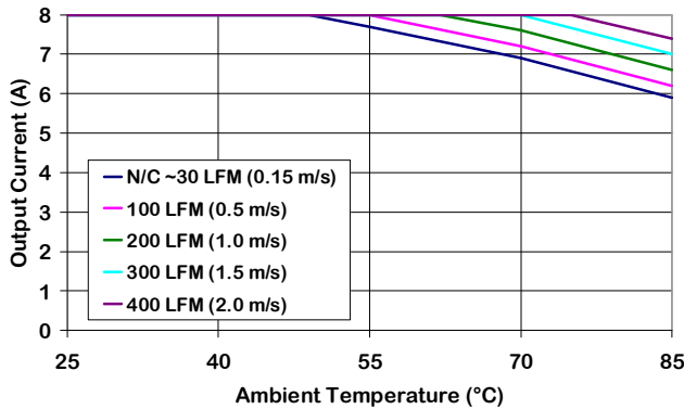
Figure 7. Output Current Derating vs Ambient Temperature & Airflow (converter mounted vertically with air flowing from Vout to Vin, Vin = 48 V.)
