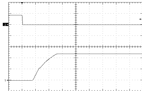
Figure 12. Startup Waveform via Enable Pin (5V/div), time scale 10mS/div. Vin=Vin_nom, full resistive load + 4700uF (negative enable.)
