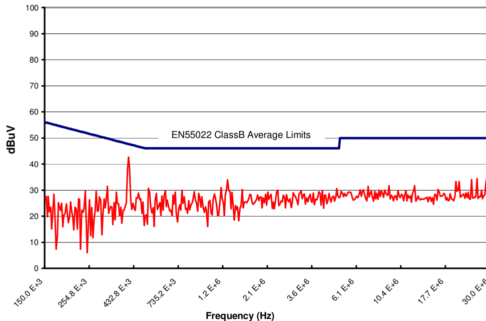
Figure 18. CPE8B48N Conducted Emissions using above specified input filter. Vin = 48V, Full Resistive Load
