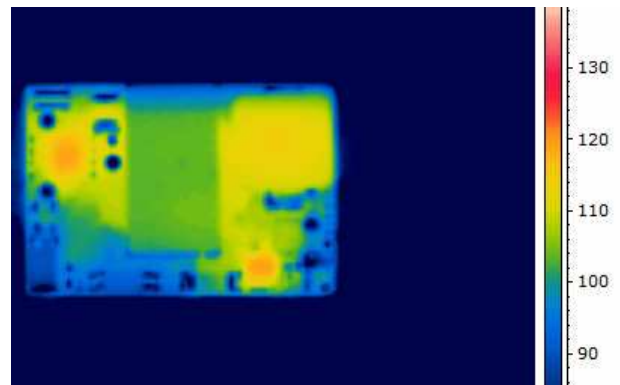
Figure 8. Thermal Image of CPT8A18 (8A output, 70C Ambient, 200lfm airflow, Vin = 18V, airflow from pin 3 to pin 1, T max = 117°C)
