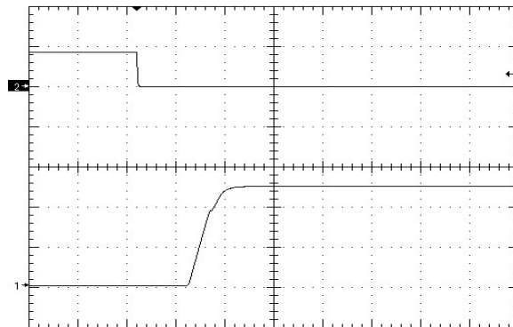
Figure 12. Startup Waveform via Enable Pin (2V/div), time scale 10mS/div. Vin=Vin_nom, full resistive load + 4700uF (negative enable.)
