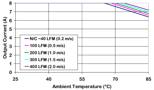
Figure 6. Output Current Derating vs Ambient Temperature & Airflow (converter mounted vertically with air flowing from pin 3 to pin 1, Vin = 12 V.)
