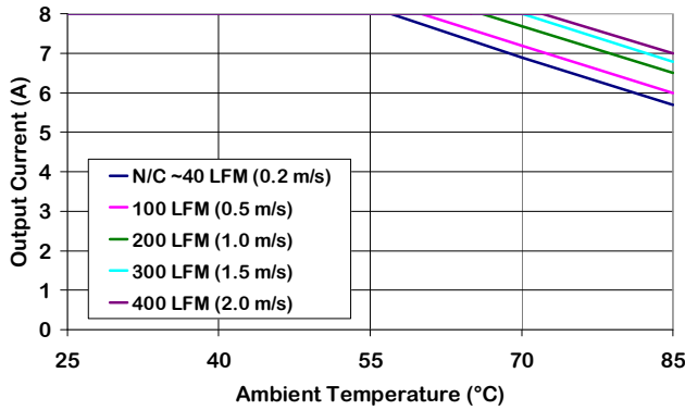
Figure 7. Output Current Derating vs Ambient Temperature & Airflow (converter mounted vertically with air flowing from pin 3 to pin 1, Vin = 24 V.)
