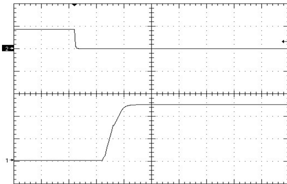
Figure 11. Startup Waveform via Enable Pin (2V/div), time scale 10mS/div. Vin=Vin_nom, full resistive load (negative enable.)
