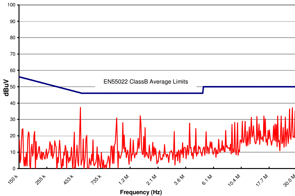
Figure 19. CPT15F36N Conducted Emissions using above specified input filter. Vin = 48V, Full Resistive Load (24Vin - subtract 2dB from peaks)
