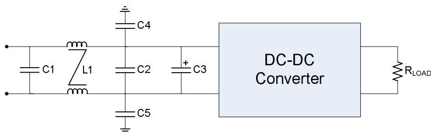
Figure 16. EMI Filter
