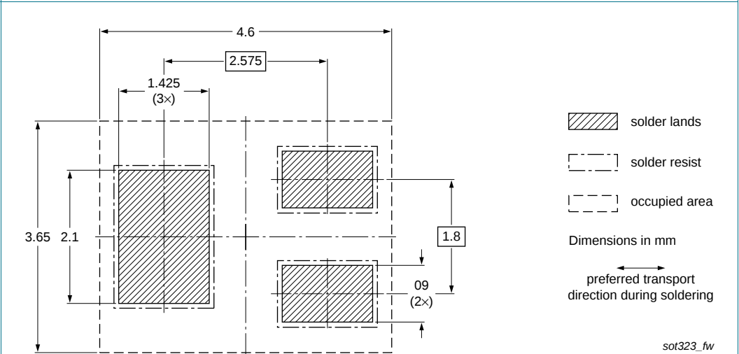
Fig 21. Wave soldering footprint PDTA143EU (SOT323/SC-70)
