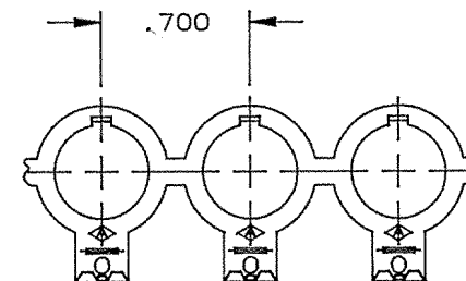
FABRICATED TERMINAL STRIP
