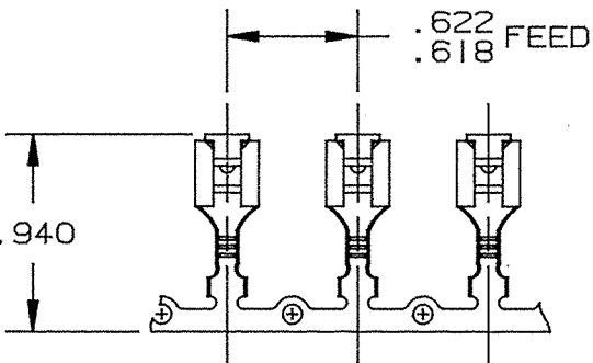
FABRICATED TERMINAL STRIP SCALE 1:1
