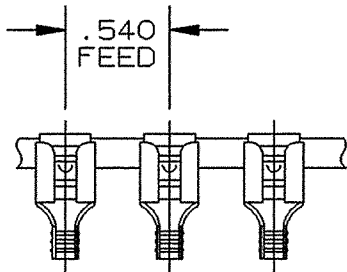
FABRICATED TERMINAL STRIP
