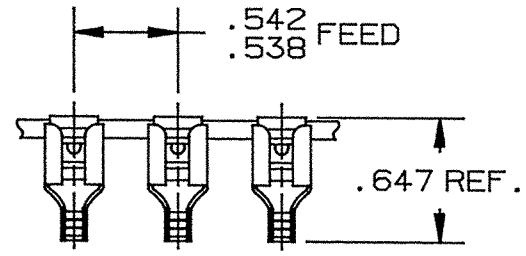
FABRICATED TERMINAL STRIP SCALE: FULL
