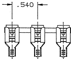
FABRICATED TERMINAL STRIP SCALE 1=1
