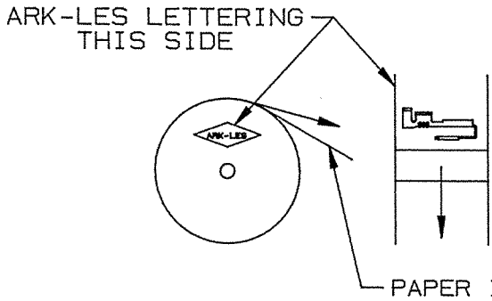
FIGURE 1 STANDARD REELING (I.E. 3800H74A-5)
