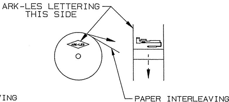
FIGURE 2 REVERSE REELING (I.E. 3800H74A-4R)
