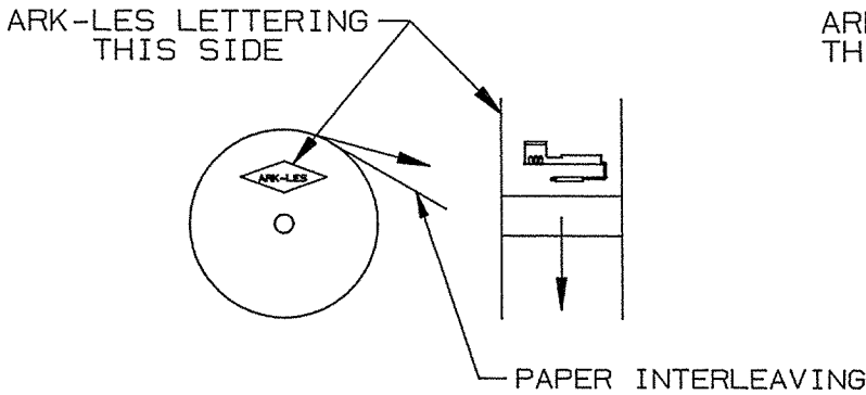
FIGURE 1 STANDARD REELING (I.E. 3800H74A-2)
