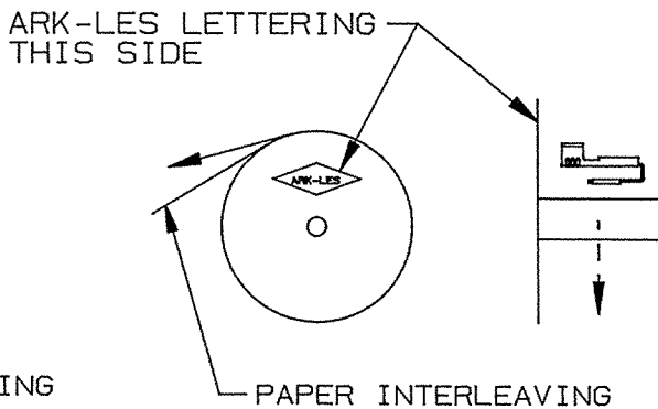
FIGURE 2 REVERSE REELING (I.E. 3800H74A-2R)
