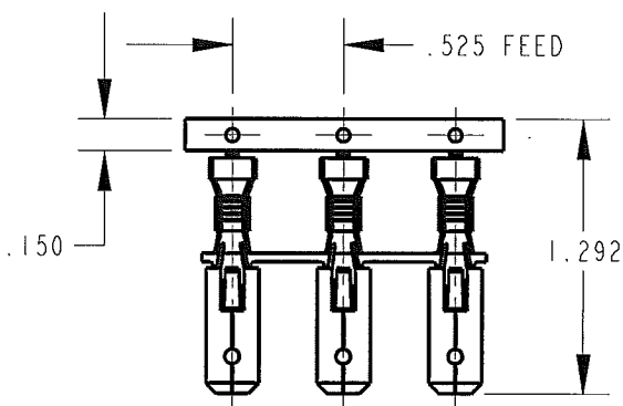
FABRICATED TERMINAL STRIP SCALE: FULL
