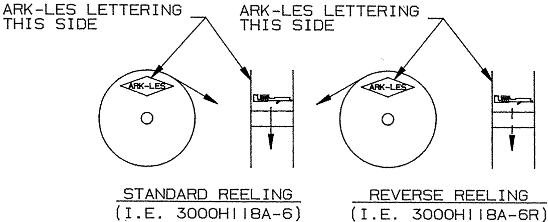
REELING DIAGRAMS
