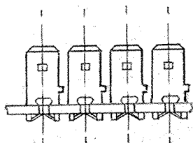
FABRICATED TERMINAL STRIP SCALE: FULL
