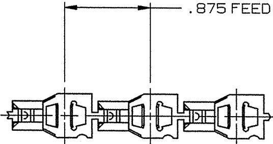
FABRICATED TERMINAL STRIP SCALE: FULL
