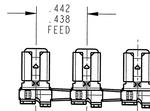
FABRICATED TERMINAL STRIP SCALE 2:1
