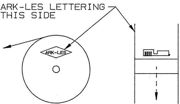
FIGURE 2 REVERSE REELING (I.E. 3700H103A-2R)
