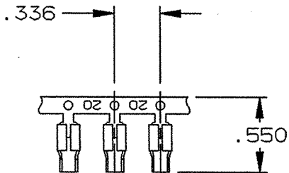
FABRICATED TERMINAL STRIP
