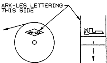
FIGURE 2 REVERSE REELING (I.E. 3650H 2AR)
