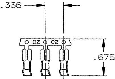
FABRICATED TERMINAL STRIP
