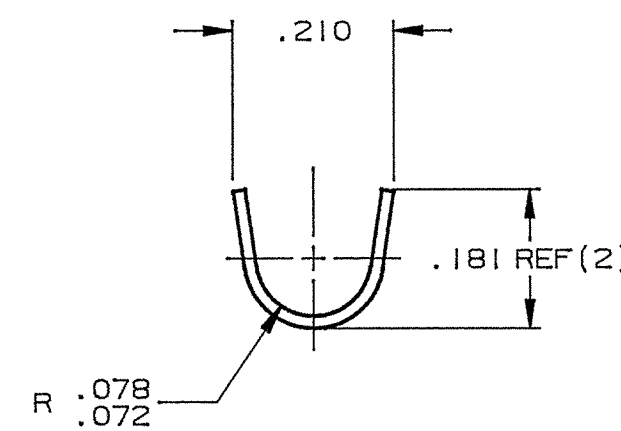
INSULATION GRIP
