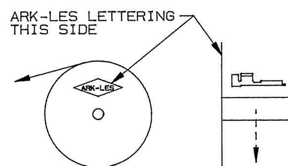
REVERSE REELING (I.E. 3000H63E-5R)
