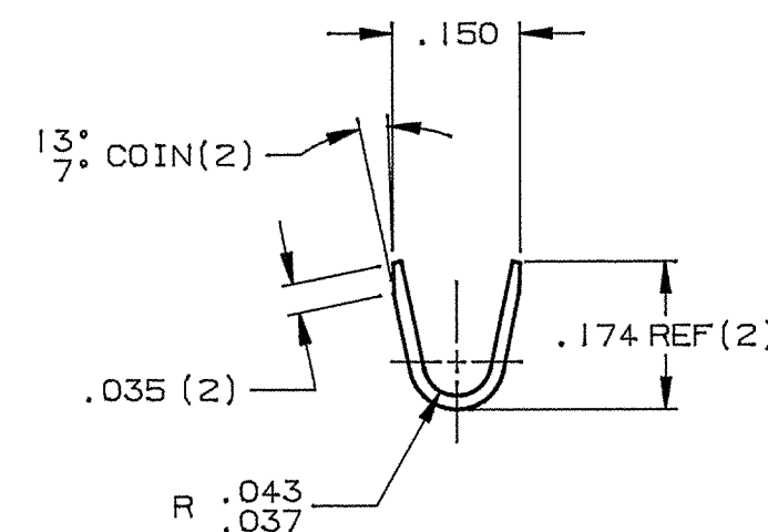
WIRE GRIP
