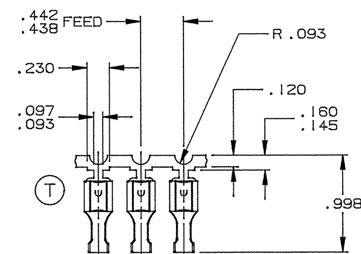
FABRICATED TERMINAL STRIP
