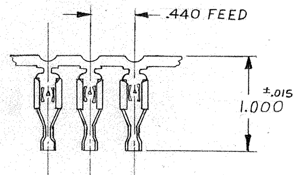
FABRICATED TERMINAL STRIP
