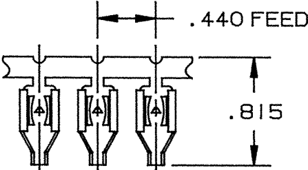
FABRICATED TERMINAL STRIP
