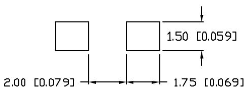
RECOMMENDED SOLDER PAD LAYOUT
