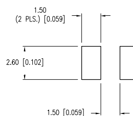
B RECOMMENDED SOLDER PAD LAYOUT
