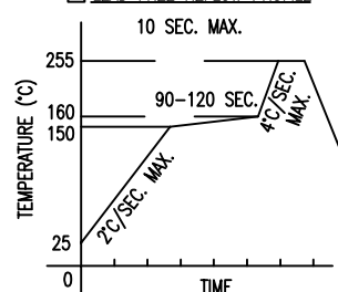
② LEAD FREE REFLOW PROFILE
