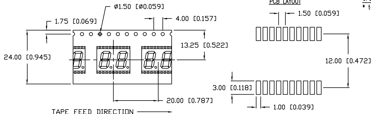
PCB LAYOUT
