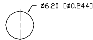
PANEL CUTOUT
