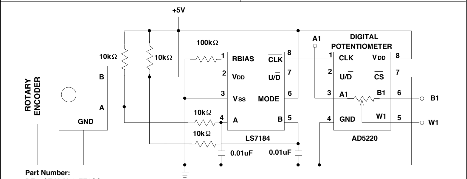
FIGURE 7. Rotary Encoder Control of Digital Potentiometer
