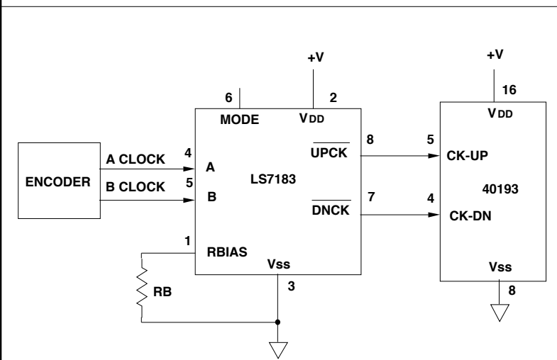
FIGURE 6A. TYPICAL APPLICATION FOR LS7183 IN x4 MODE
