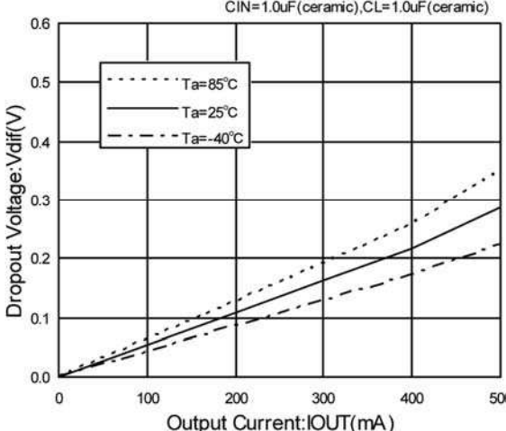
XC6210 (VOUT:2.5V)
