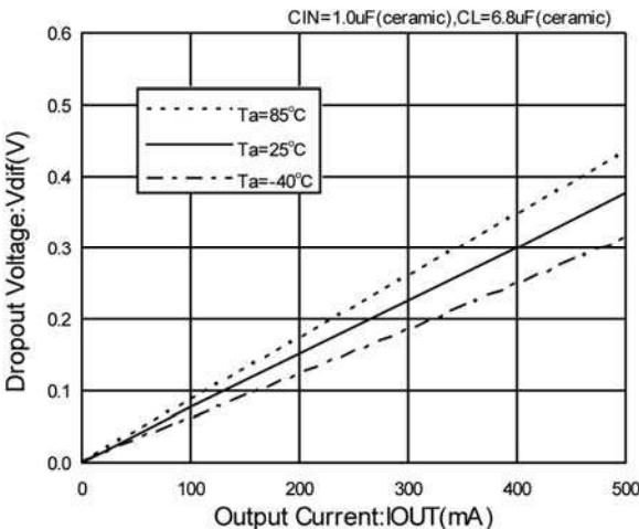
XC6210 (VOUT:1.5V)
