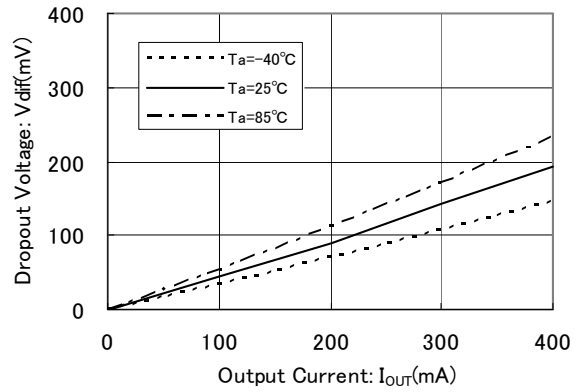
XC6601B121MR ( V_{gs}^{(*1)}=2.4\text{V} )
