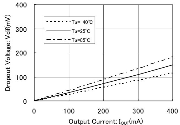
XC6601B121MR ( V_{gs}^{(*1)}=3.8\text{V} )
