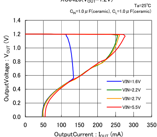
XC6420( V_{OUT}=1.2V )
