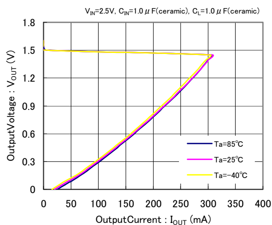
XC6415( V_{OUT}=1.5V )
