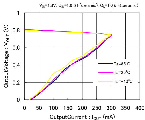
XC6415( V_{OUT}=0.8V )
