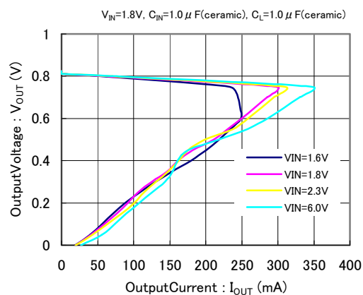
XC6415( V_{OUT}=0.8V )
