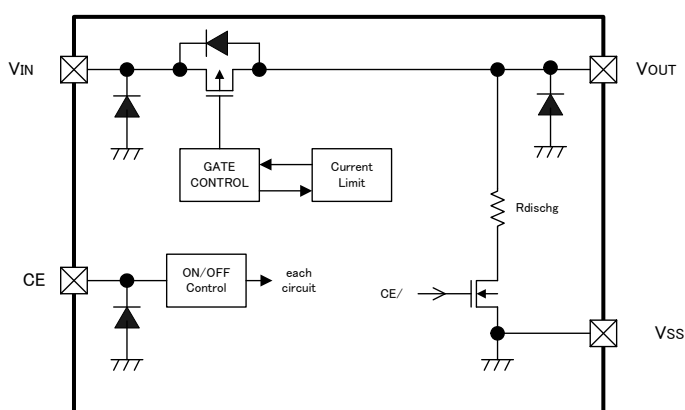
XC8102AA Series
