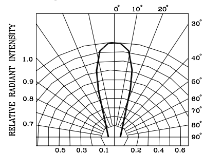
Fig.6 RADIATION DIAGRAM
