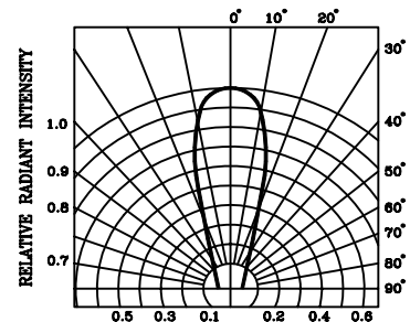
Fig.6 RADIATION DIAGRAM
