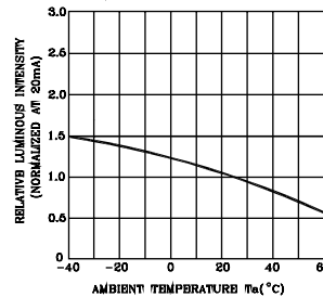
Fig.4 RELATIVE LUMINOUS INTENSITY VS. AMBIENT TEMPERATURE
