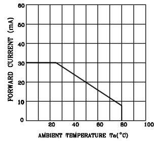
Fig.2 FORWARD CURRENT DERATING CURVE
