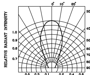
RADIATION DIAGRAM
