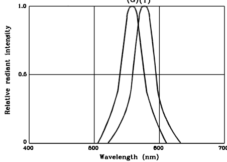
Fig.1 Relative intensity vs. wavelength (G)(Y)
