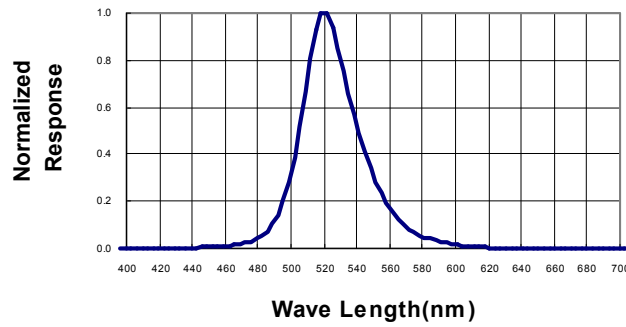
Spectral Radiance (Peak @ 520 nm)
