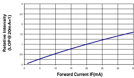
Relative Luminous Intensity vs Forward Current
