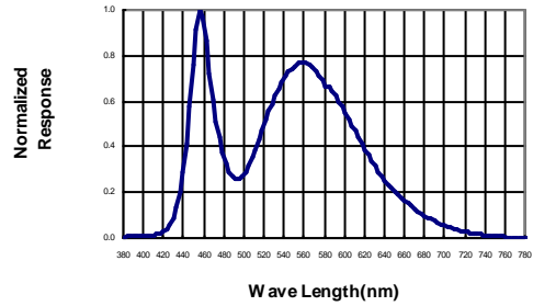
Spectral Radiance
