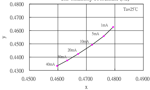
Forward Current VS. Chromaticity coordinate ( \lambda_d )
