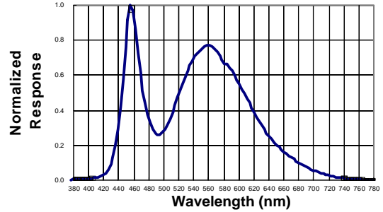
Spectral Radiance
