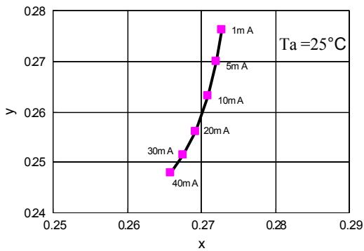
Forward Current vs. Chromaticity Coordinates
