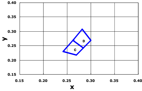
CIE 1931 Chromaticity Diagram
