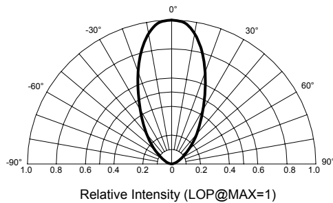
Beam Pattern
